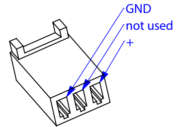
Connector Molex 22-01-3037
